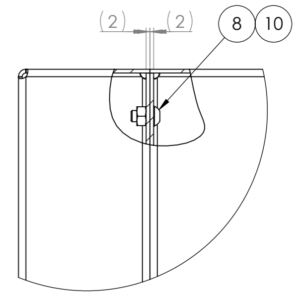
DETAIL X SCALE 1 : 2
